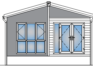
End Elevation (Lounge)
