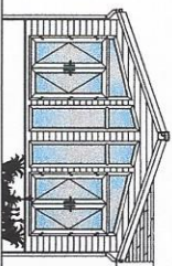
END ELEVATION (LOUNGE)
